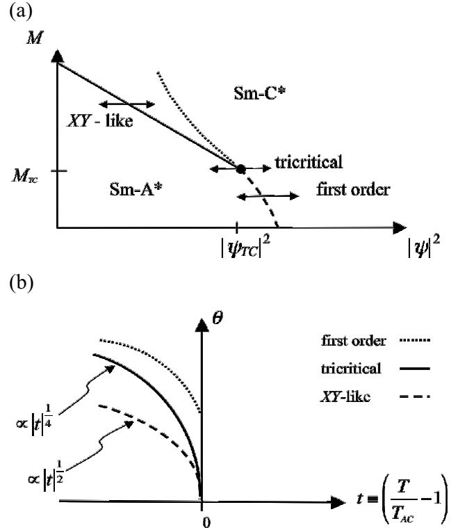
FIG. 2. (a) The phase diagram in |\psi|^2 – M space near the tricritical point (|\psi_{TC}|^2, M_{TC}) . The quantity M is a measure of how much orientational order the system possesses and for de Vries materials is effectively athermal. The quantity |\psi| is a measure of the strength of the layering. It is a monotonically decreasing function of temperature so that for a given material, decreasing the temperature corresponds to moving horizontally from left to right. The solid line represents the continuous Sm-A*–Sm-C* boundary while the dashed line represents the first-order Sm-A*–Sm-C* boundary. These two boundaries meet at the tricritical point (|\psi_{TC}|^2, M_{TC}) . The dotted line indicates the region in which the behavior crosses over from XY like to tricritical. The region in which the behavior is XY like shrinks to zero as the tricritical point is approached. At the tricritical point the slopes of the first-order and continuous Sm-A*–Sm-C* boundaries are equal but the curvatures are not. Also shown, as double ended arrows, are the three distinct classes of transitions: XY like, tricritical, and first order. (b) The tilt angle \theta as a function of reduced temperature t \equiv (1 - \frac{T}{T_{AC}}) near the Sm-A*–Sm-C* transition temperature T_{AC} , i.e., for |t| \ll 1 . Upon entry to the Sm-C* phase the growth of the tilt angle scales like |t|^{1/2} for a mean-field XY-like transition. For a tricritical transition it scales like |t|^{1/4} and is thus more rapid. For a first-order transition there is a jump in the tilt angle upon entry to the Sm-C* phase.
