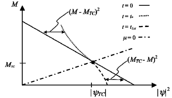
FIG. 5. The t=0 (solid), \mu=0 (dashed-dotted), t=t_* \propto -(M - M_{TC})^2 (dotted), and t=t_{1st} \propto (M_{TC} - M)^2 (dashed) loci in |\psi|^2 - M space. The corresponding phase diagram is shown in Fig. 2(a). The continuous transition occurs for \mu \geq 0 and at t=0 . Thus, the tricritical point (|\psi_{TC}|^2, M_{TC}) is located at the intersection of the t=0 and \mu=0 loci. The first-order Sm-A*–Sm-C* transition occurs for \mu < 0 and at t > 0 . The horizontal separation between the first-order boundary and the extrapolated continuous boundary scales like (M_{TC} - M)^2 . Similarly, the separation between the continuous boundary and the tricritical crossover region at t_* scales like (M - M_{TC})^2 . The negative slope of the Sm-A*–Sm-C* phase boundary implies that the smaller the value of M , the larger the value of |\psi| at which the Sm-A*–Sm-C* transition occurs. This is consistent with the observation that de Vries smectics generally have such unusually weak orientational order that their stabilization requires strong layering order, perhaps via microsegregation.
